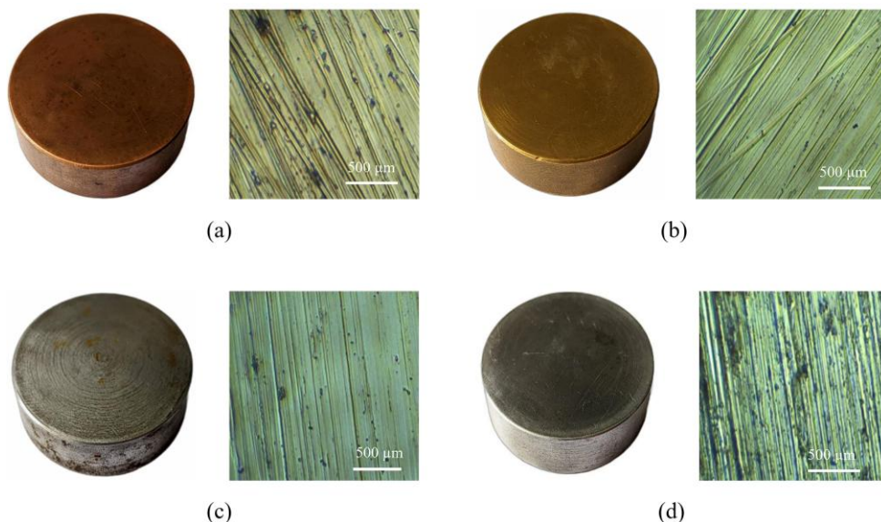
Figure 6. Specimen and surface topography (@100x magnification) for testing purpose (a) Copper, (b) Brass, (c) Steel, and (d) Aluminum.
