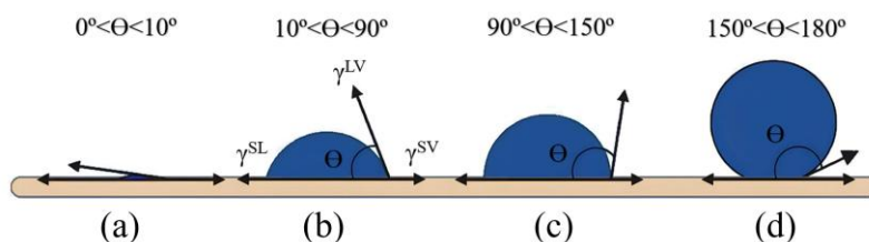
Figure 1. Illustration of contact angles on a smooth homogeneous solid surface.
